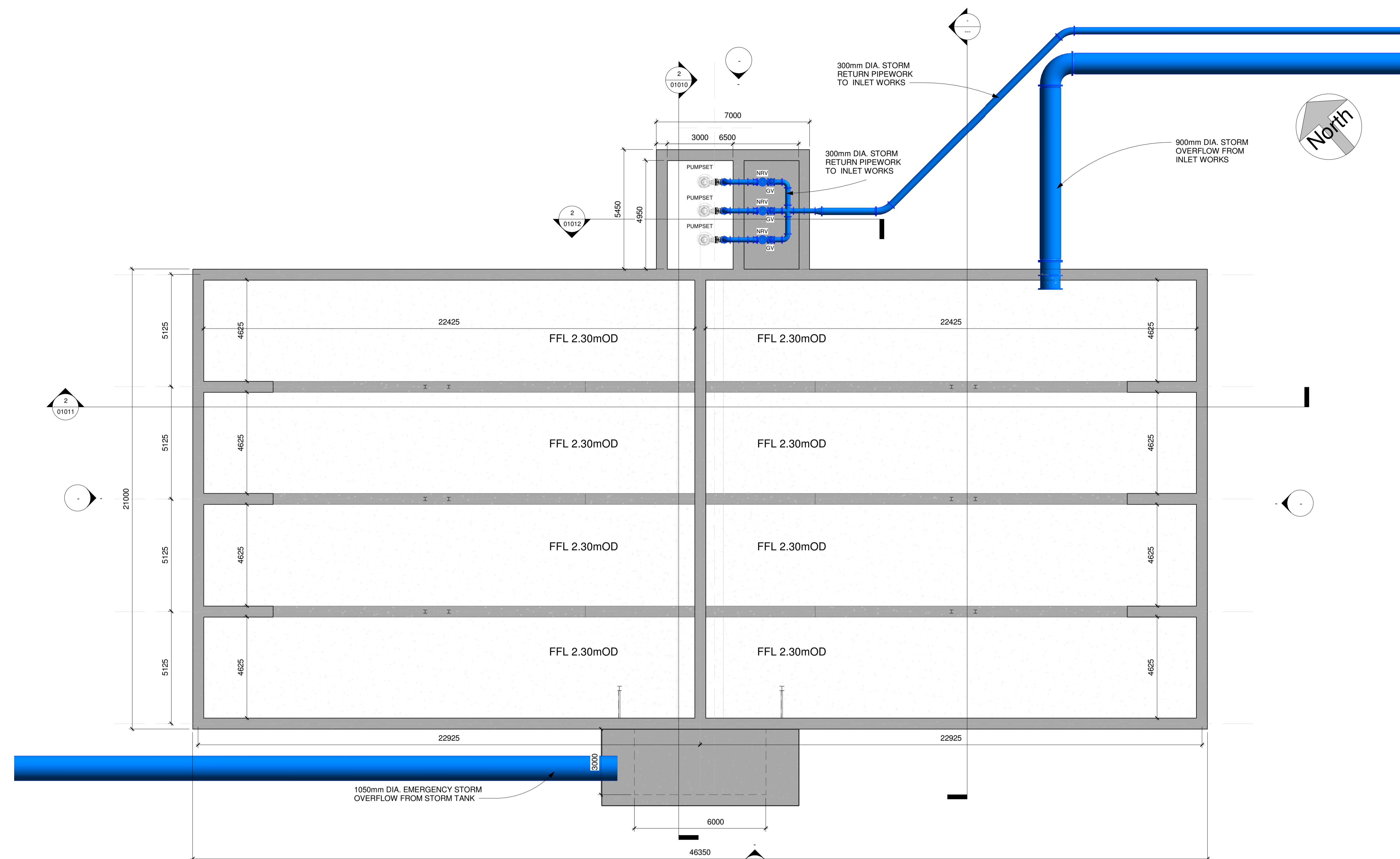
1 Stormwater Storage Tank Floor Plan 1 : 100
